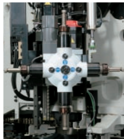
4-Station Tapping Unit (Option)
